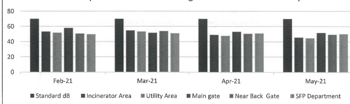
Trend Analysis of Noise Level at Night Time Feb-2021 to May-2021
